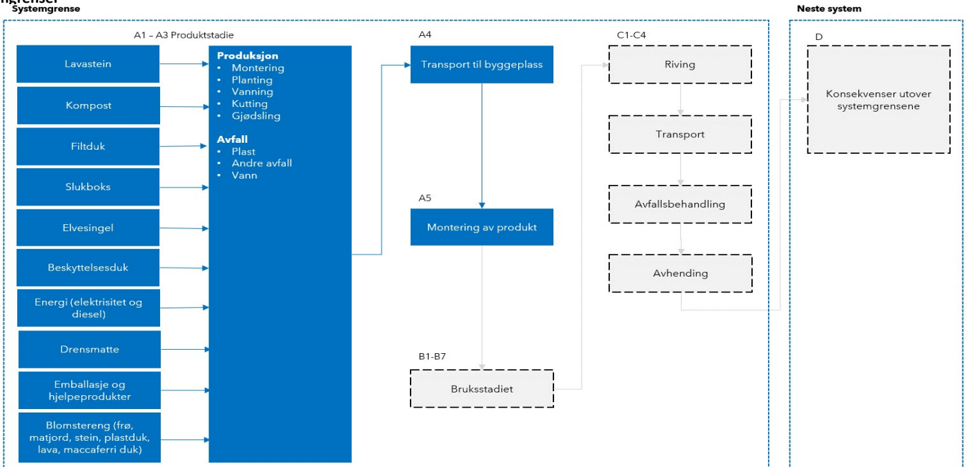
Figur 1: Systemgrenser
